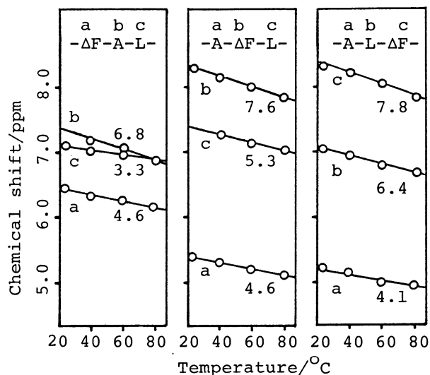
Fig. 3. Temperature dependence of amide protons of the major conformer in DHP (in CDCl 3 ). Numbers on the lines refer to 10^3 \times temperature efficient in ppm °C -1 .
