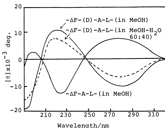
Fig. 2. CD spectra of the diastereomers ( \Delta^1 -DHP) in MeOH and in a mixture of MeOH-H 2 O.
