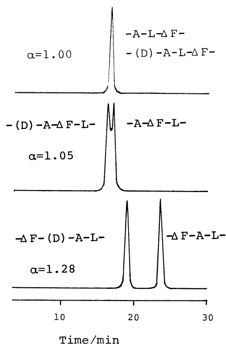
Fig. 1. Separation of \Delta^3 -, \Delta^2 -, and \Delta^1 -DHP containing racemic alanine residue. Column: 250 mm x 4.5 mm, RP-18.
